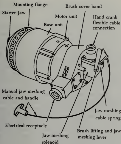
FIGURE 5-6. Combination inertia starter.
